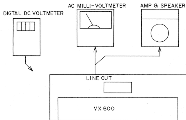
Fig. 4-25 Instrument connection
