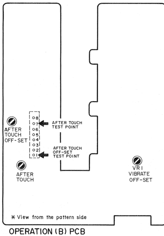
Fig. 4-26 Adjustment points of the OPERATION (B) PCB.
