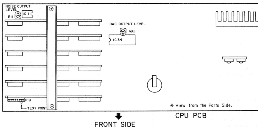
Fig. 4-27 Adjustment points of the CPU PCB
